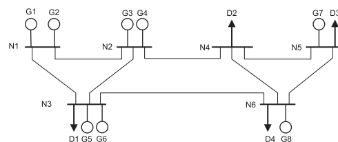
Fig. 1. Six-bus test system.
